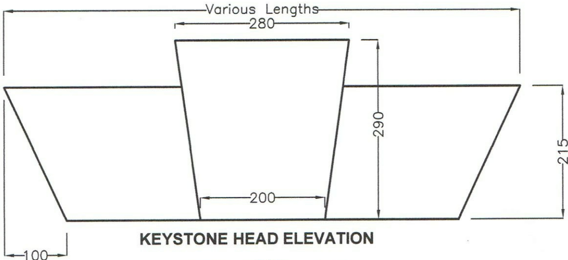
HEAD PROFILE
