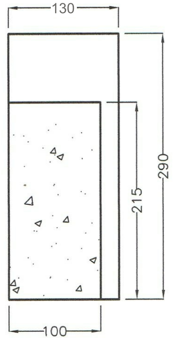
HEAD PROFILE
